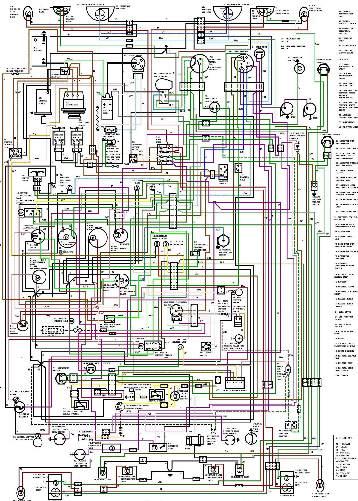
Typical wiring diagram, later N. American models
